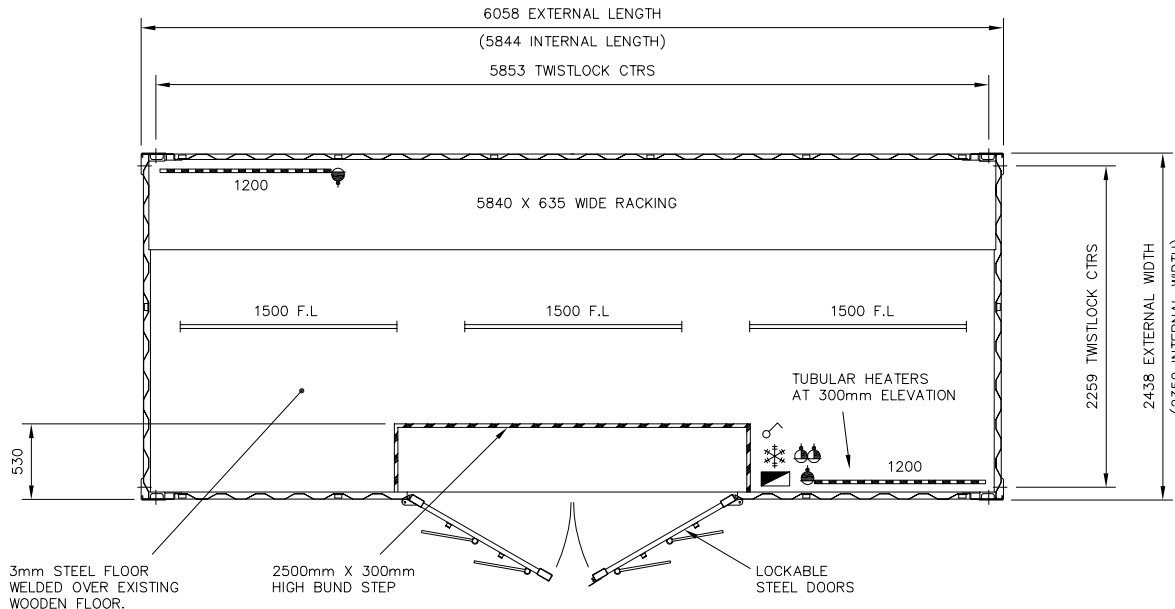
SECTIONAL PLAN
