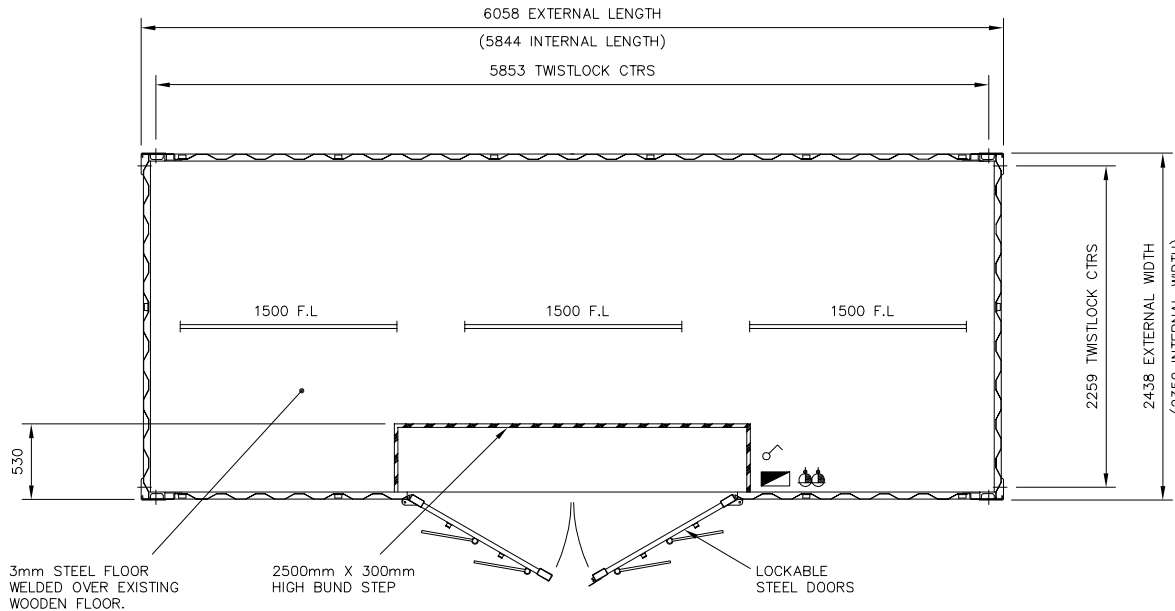
SECTIONAL PLAN
