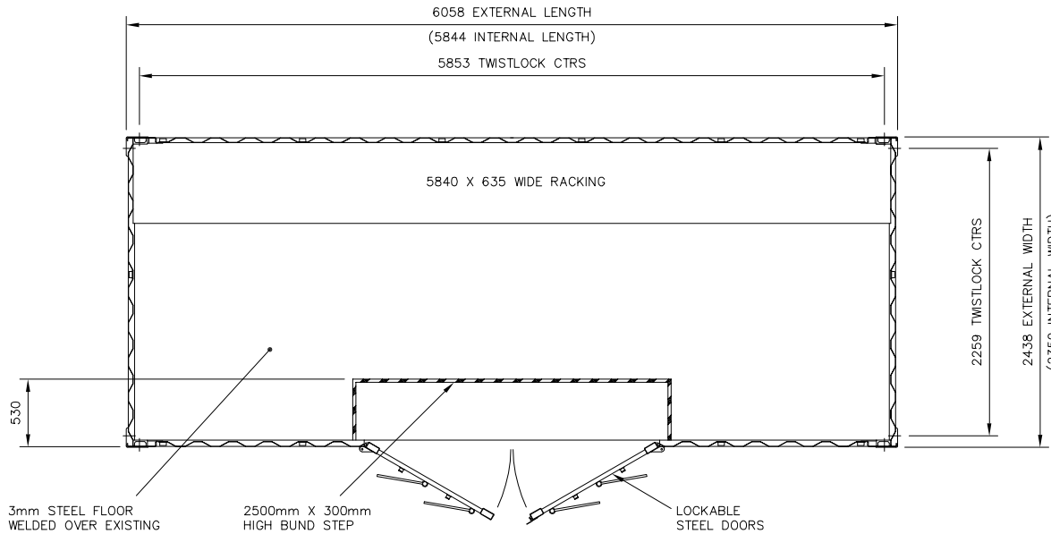
SECTIONAL PLAN
