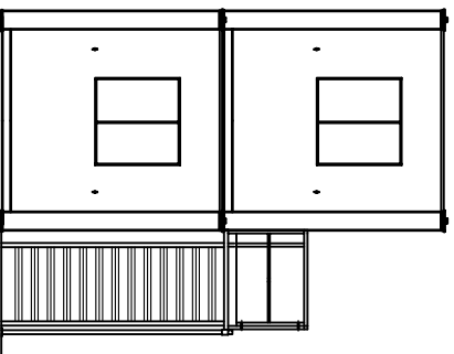
LEFT ELEVATION
