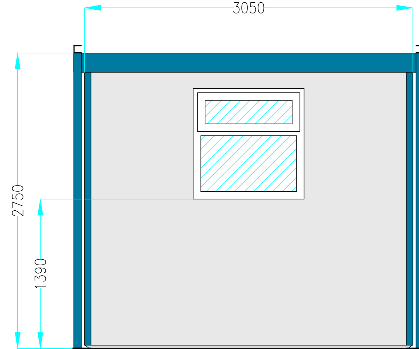
SIDE ELEVATION "C"
