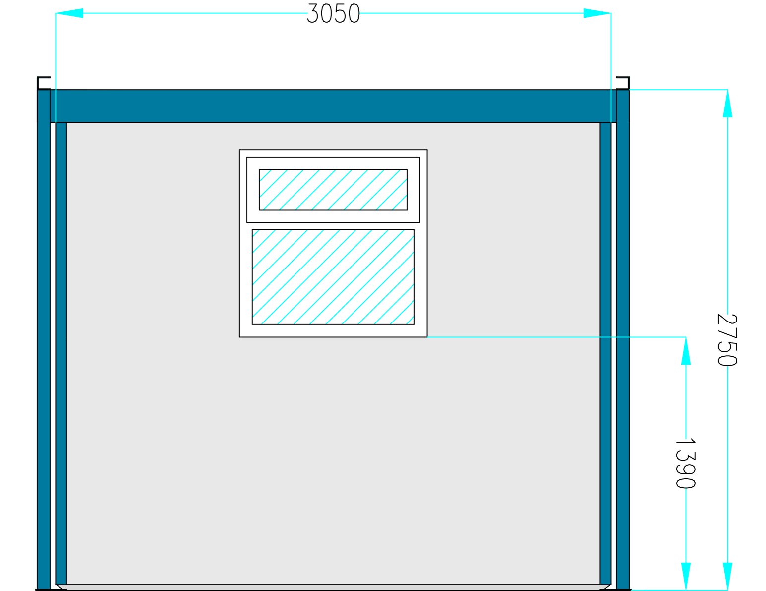
SIDE ELEVATION "D"
