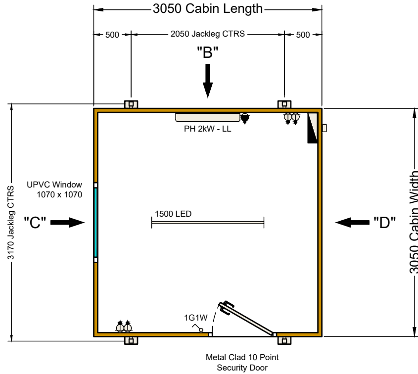
SECTIONAL PLAN
