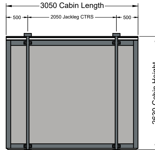
SIDE ELEVATION "B"
