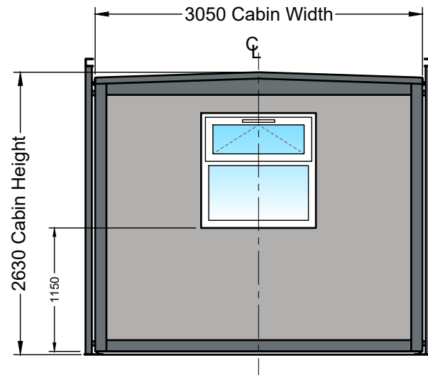
SIDE ELEVATION "C"
