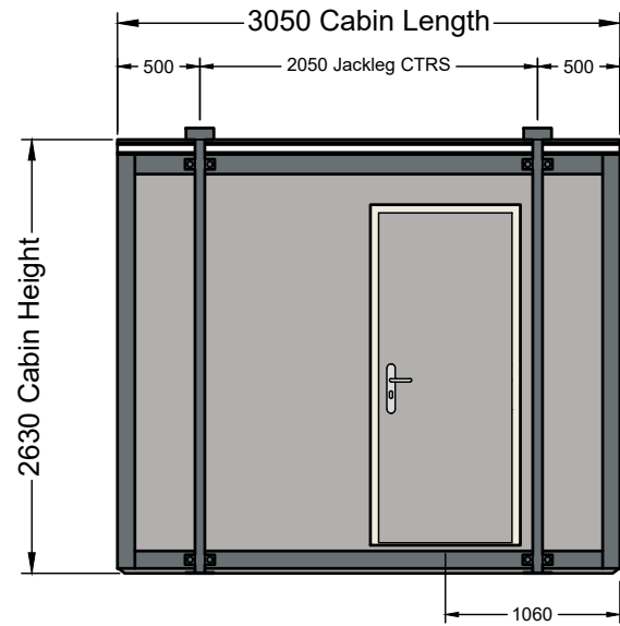
SIDE ELEVATION "A"
