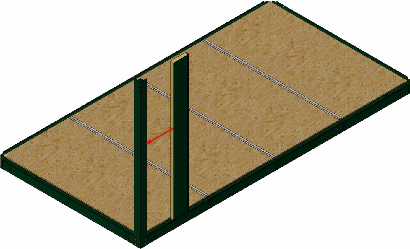
4. After the corner profile is fixed, the small panel for the side part is placed.
